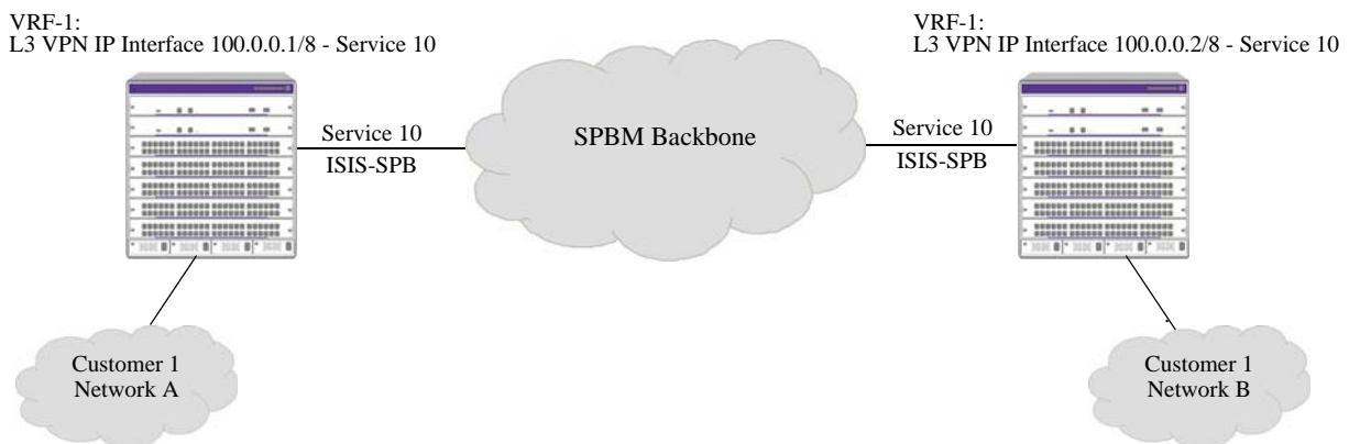
Figure 7: IPv4 L3 VPN Service-Based Interface (No Loopback)
