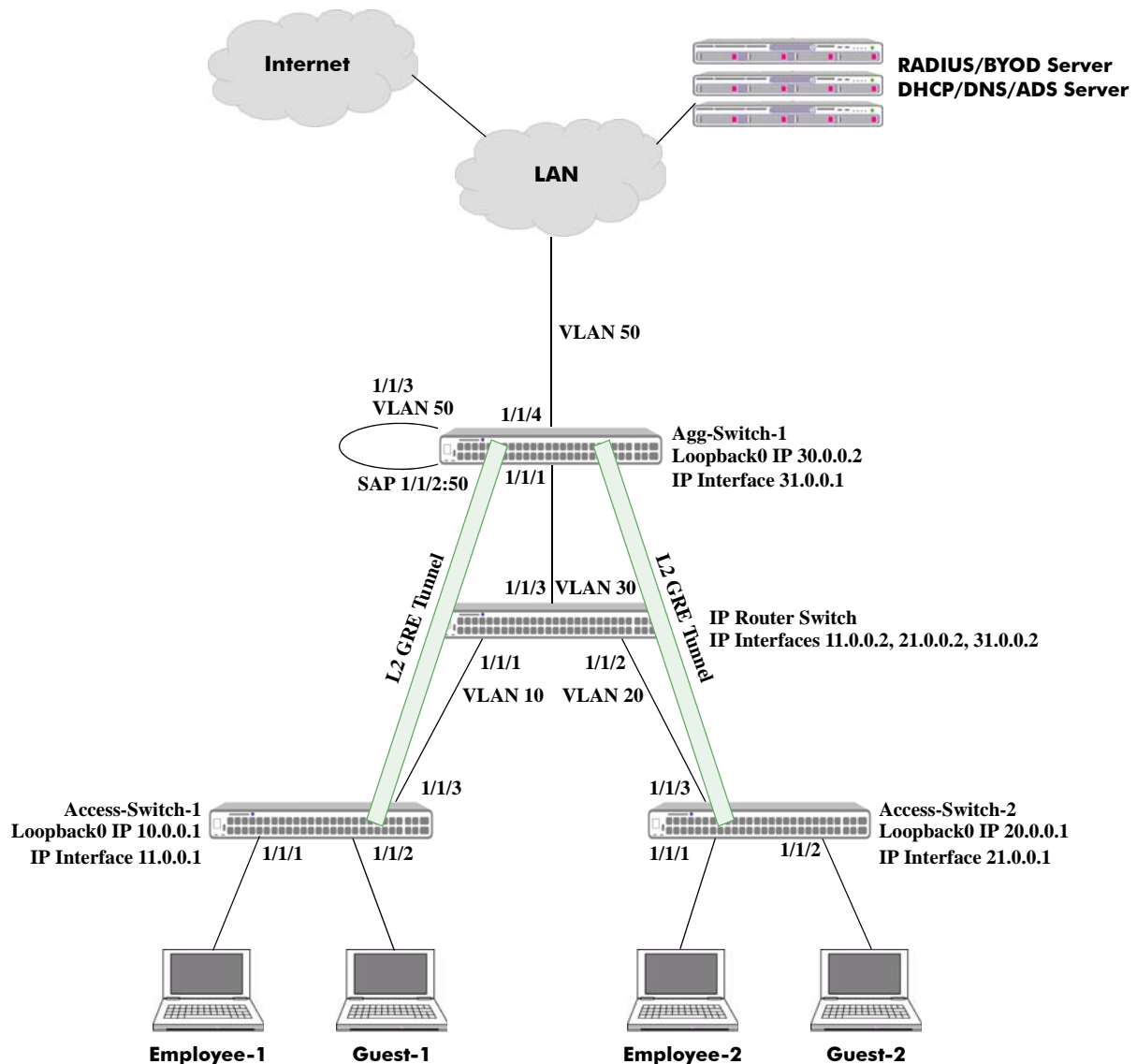
OmniSwitch L2 GRE Tunneling Configuration Example
